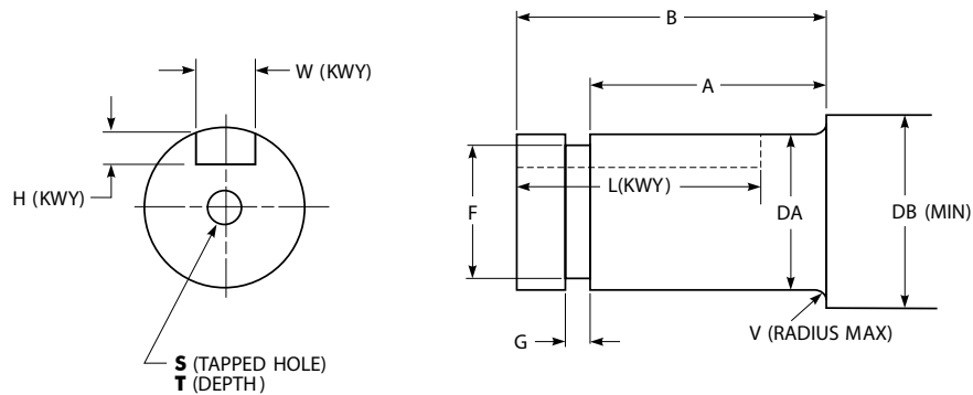
FIGURE 1 (SIZES M1130-M1190)
