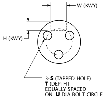
FIGURE 2 (SIZES M1200-M1210)
